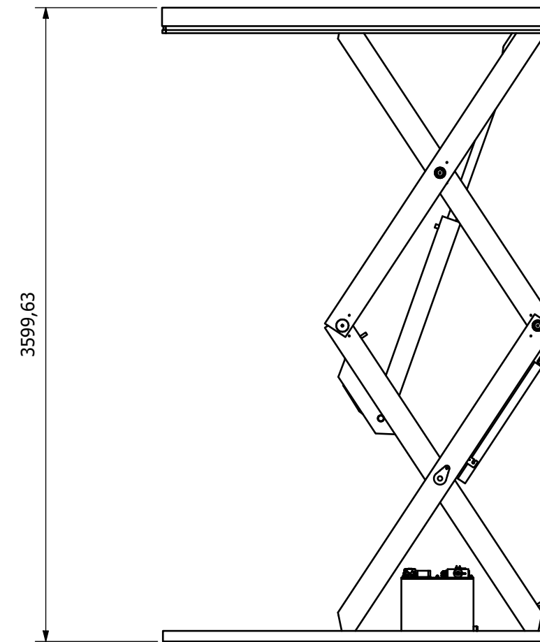
Over lift ( 1:30 )
